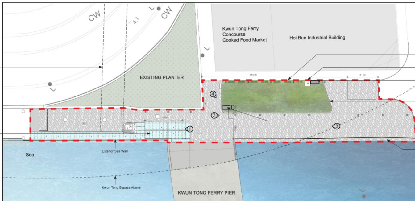
Roof Plan
