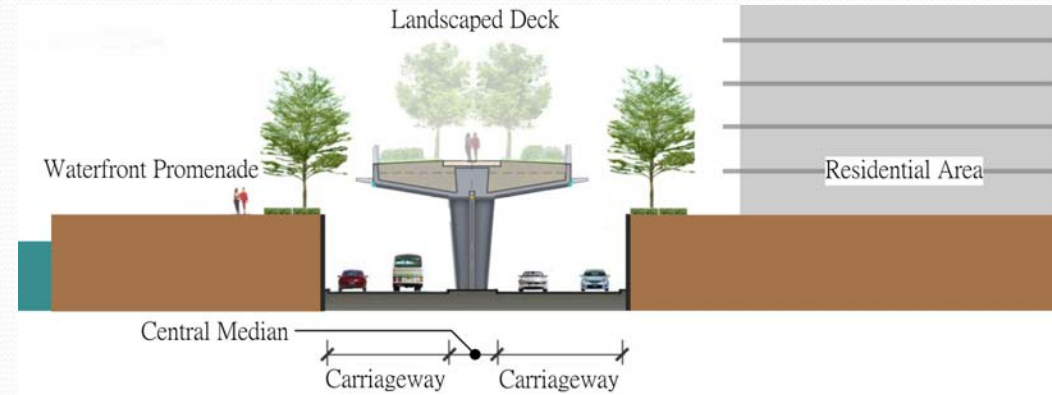
Cross-section C-C Landscaped Deck at Depressed Road Section
