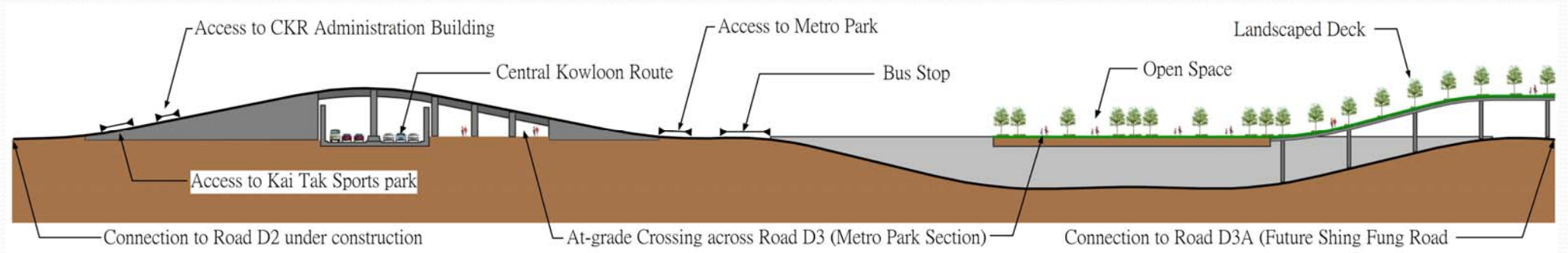
Longitudinal Section of Road D3 (Metro Park Section)
