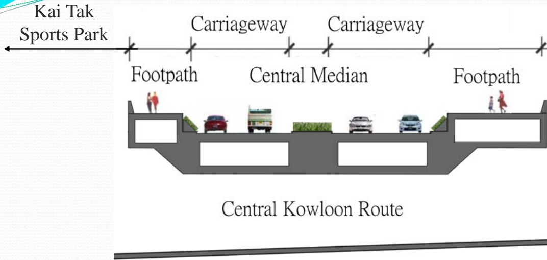
Cross-section A-A Elevated Road (Across CKR) Section
