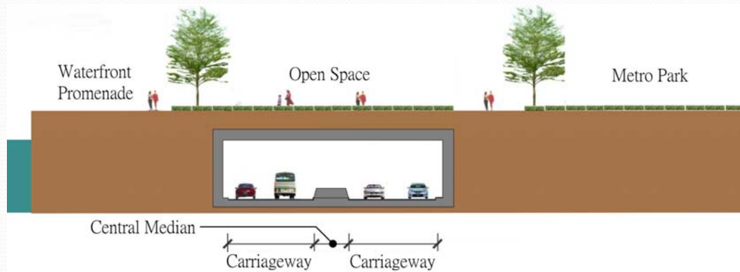
Cross-section B-B Underpass Section
