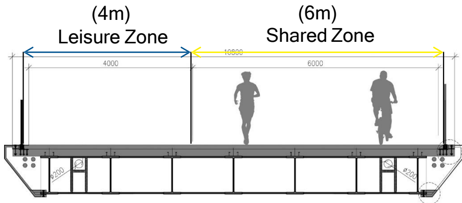
Typical Section
